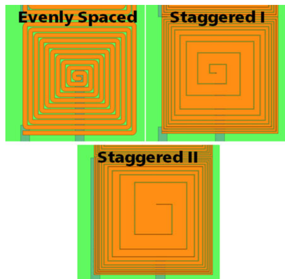
Fig. 2. Three different coil geometries for comparison.
