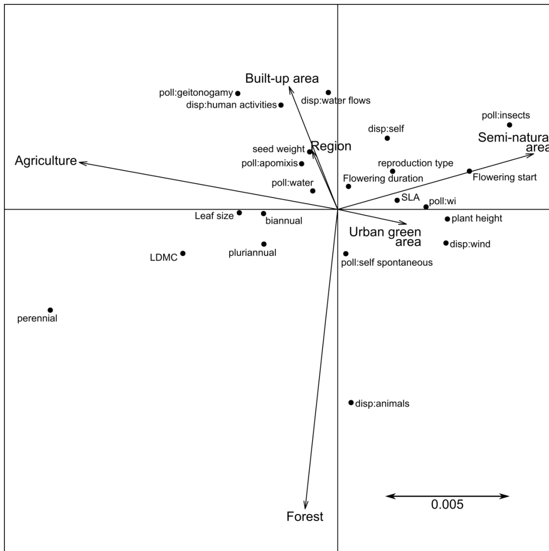
Supplementary Figure 4. Result of the second (horizontal) and third (vertical) axes of the principal component analysis applied to the coefficients of generalized least squares models (GLS). GLS was applied to species functional originalities (regional and local) with traits as explanatory variables (Supplementary Table 5). The second axis explained 8%, and the third 6% of the total variation in these coefficients. Variable names are given in Supplementary Table 5. We distinguished, in this figure, the levels of pollination that start with "poll:" from those of the dispersal mode that start by "disp:".
