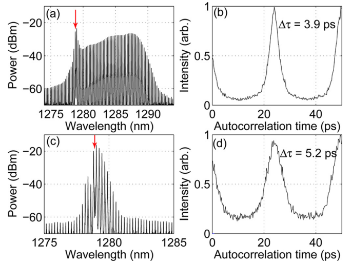
FIG. 5. (a) Optical spectrum and (b) autocorrelation trace of the PMLL with sidebands injection-locking; injection power P_{\text{inj}} = 240 \mu\text{W} . (c) Optical spectrum and (d) autocorrelation trace of the PMLL with sidebands injection-locking; injection power P_{\text{inj}} = 570 \mu\text{W} .
