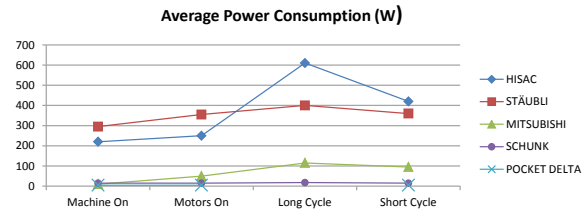
Figure 3: Average power consumption of the tested machines in different states [28].
