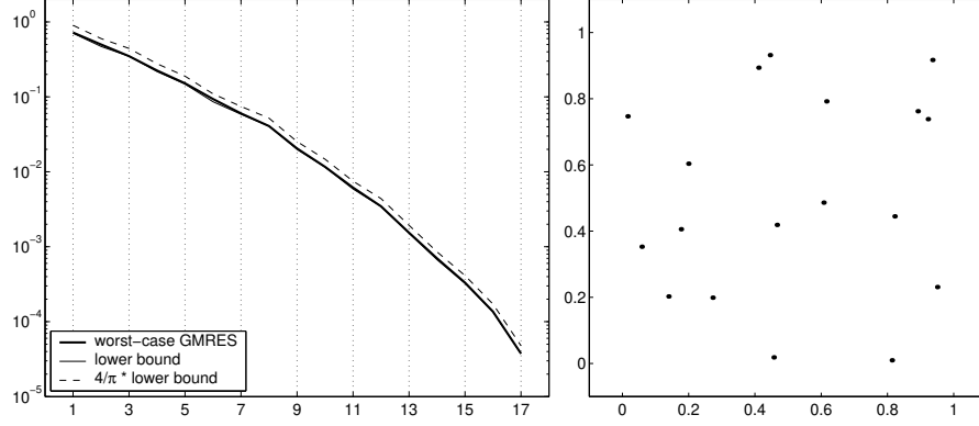
Figure 4.3: Worst-case GMRES and our bounds for random eigenvalues in the region [0, 1] \times \mathbf{i}[0, 1] .
