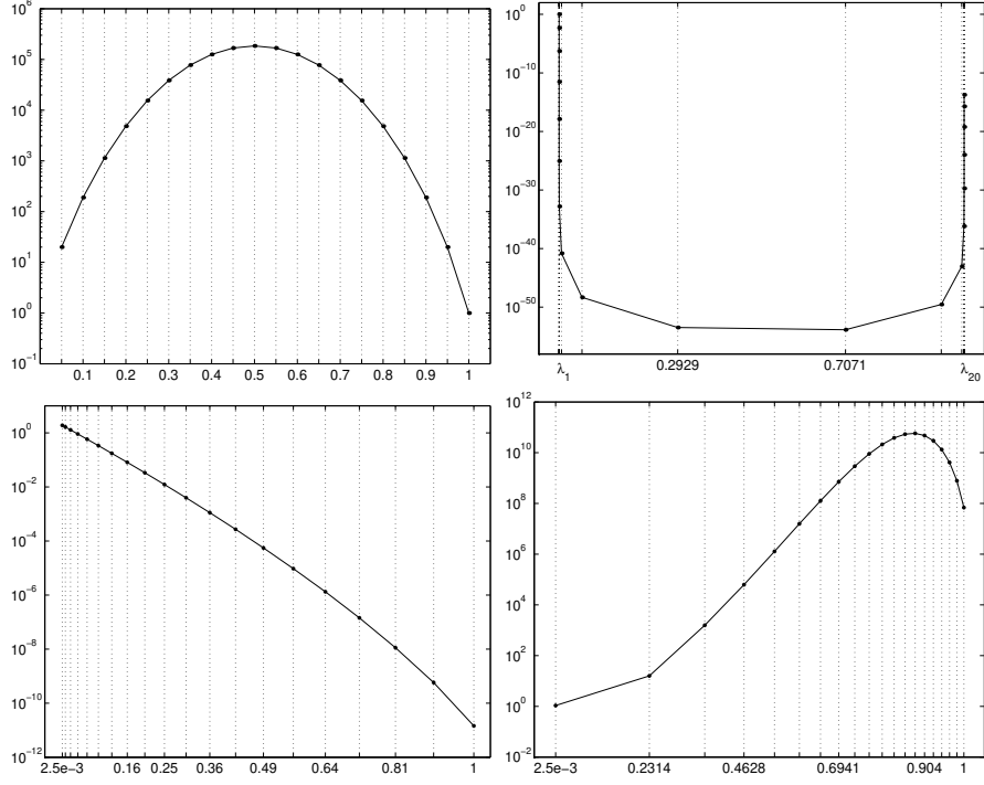
Figure 2.1: The values |l_j(0)| for example eigenvalue distributions.
