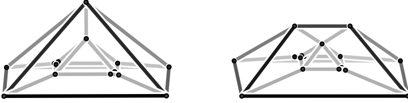
Figure 4: Schlegel diagrams (produced using polymake [5, 6] and javaview [10, 9]) illustrating two 4-polyhedra P_1 and P_2 that have the same vertex-facet incidences, but different face posets.
