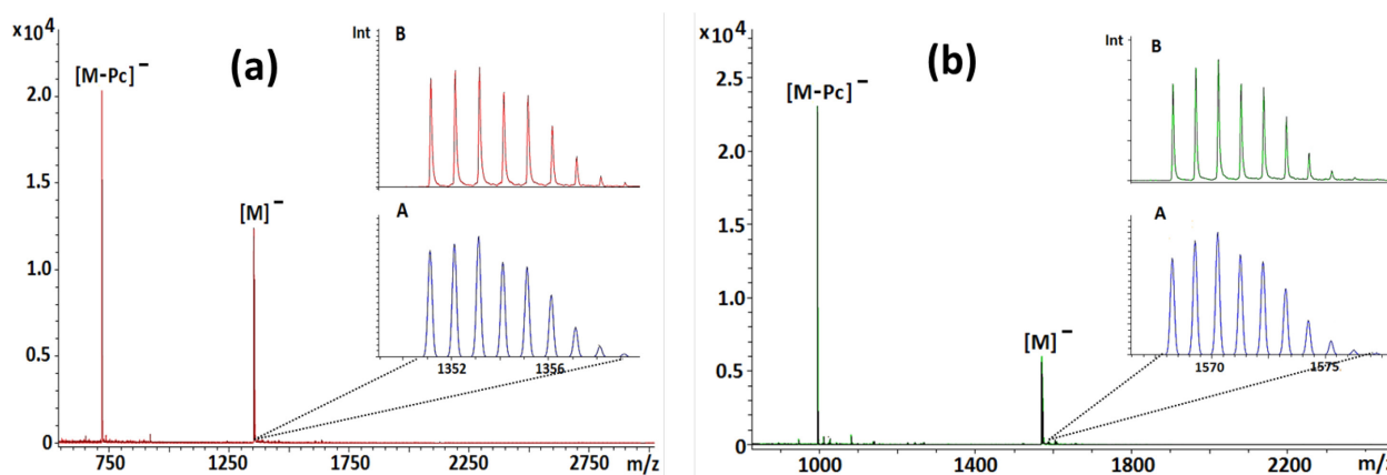
Figure 42. MALDI-TOF MS spectra (DCTB) of a) ZnPc-C 60 dyad 6 and b) its analog 19 . Inset: A) calculated isotopic pattern for the same peak, B) isotopic resolution of the MALDI-TOF main peak.
