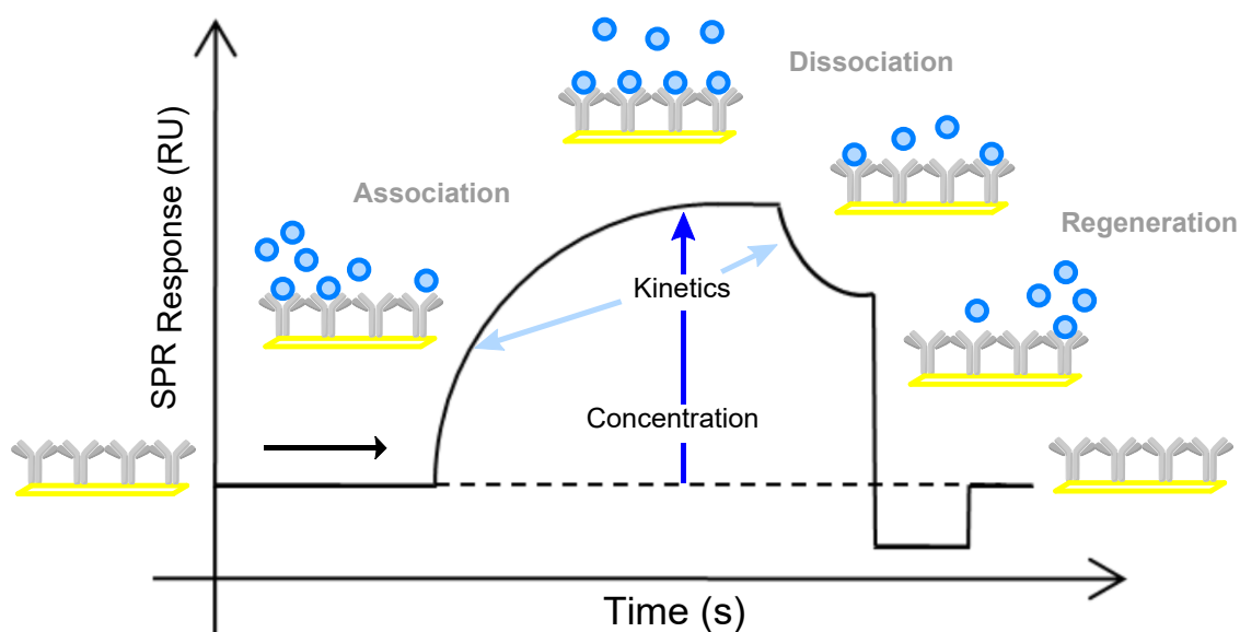
Figure 38. Typical phases and sensorgram of an SPR measurement.
