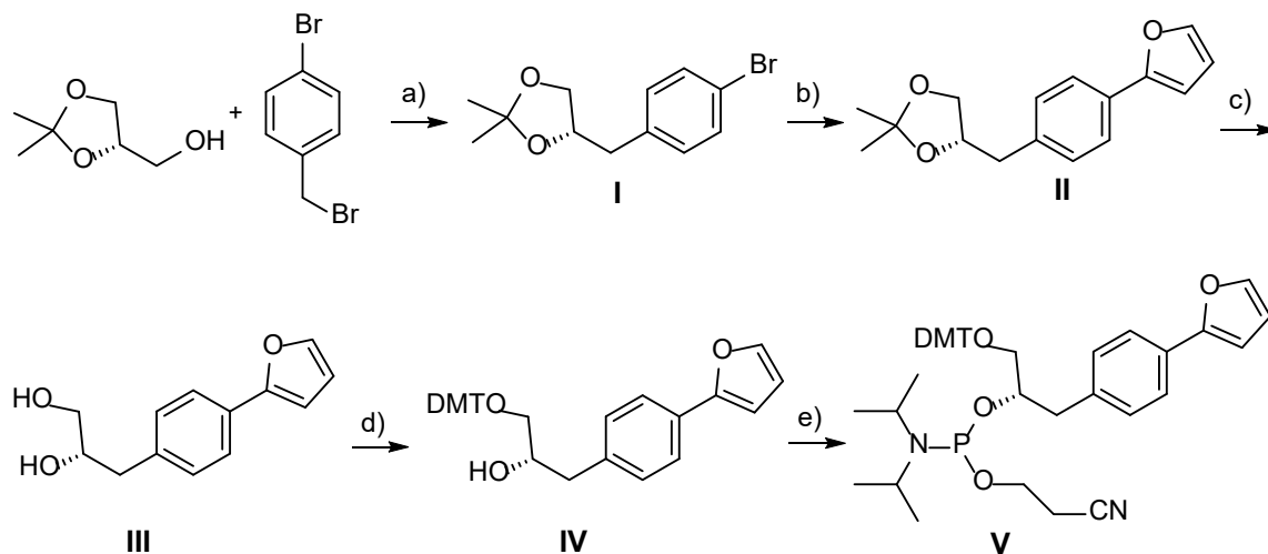
Scheme 7. Synthesis of the furan modified phosphoramidite V : a) KOH, toluene, T= 135°C, 24h. b) furan boronic acid, Pd(PPh 3 ) 4 , Na 2 CO 3 , toluene, MeOH, T= 48°C. c) HCl (4M), THF, 2h. d) DMTrCl, pyridine, T= 0°C, 3h. e) (iPrN) 2 (NCCH 2 CH 2 O)P, N,N-diisopropylammoniumtetrazolide, DCM, 0°- kT, 48h.
