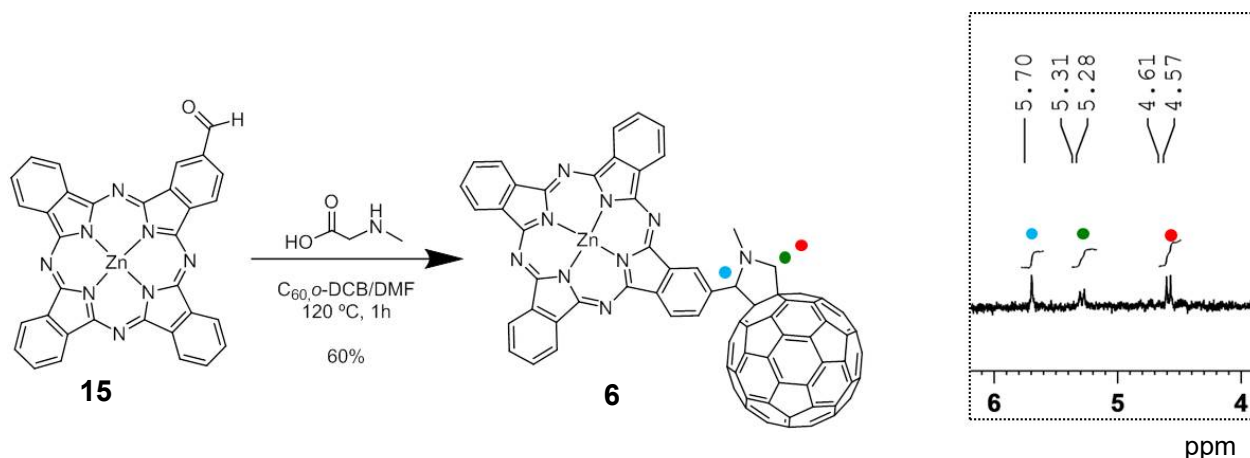
Scheme 6. Synthesis of ZnPc-C 60 dyad 6 . Inset - 1 H NMR spectrum (300 MHz, CS 2 /THF- d 8 = 1:1 vol., 25°C) with characteristic signals of the pyrrolidine unit.
