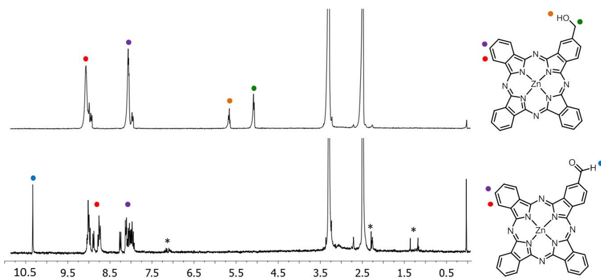
Figure 41. ^1\text{H} NMR spectra (300 MHz, \text{DMSO-}d_6 , 25^\circ\text{C} ) of hydroxymethyl-ZnPc 14 and formyl-ZnPc 15 . Color code is used for the assignment of protons and asterisks for impurities.
