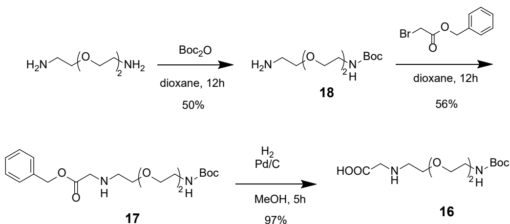
Scheme 7. Synthesis of N -functionalized glycine 16 .
