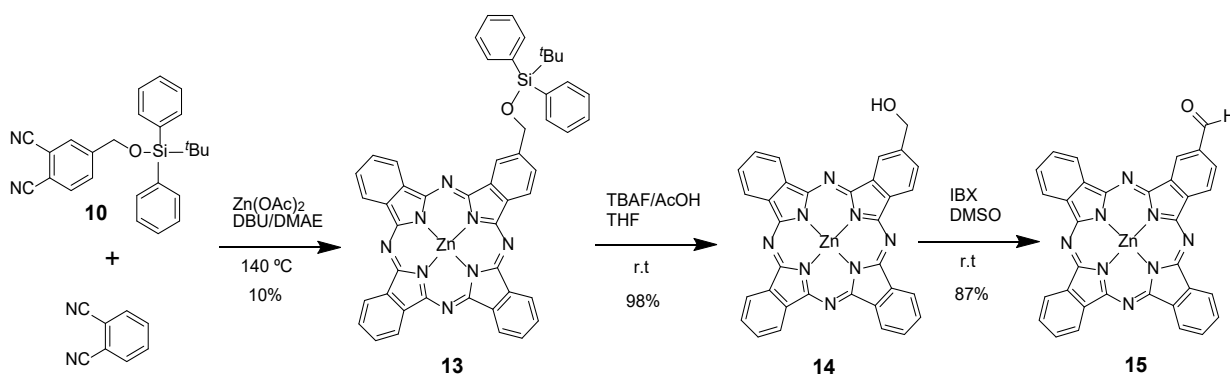
Scheme 5. Synthetic scheme leading to ZnPs 14 and 15 .
