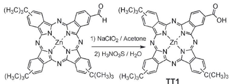
Scheme 1. Synthesis of carboxyphthalocyanine TT1. Reproduced with copyrights permissions from John WILEY-VCH Verlag GmbH & Co.
