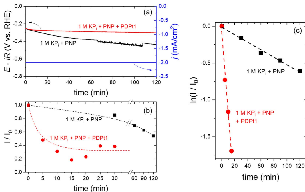
Fig. 8 Chronopotentiometry ( -2 \text{ mA cm}^{-2} , 1 M KP i buffer as catholyte, Pt foil cathode) with PNP (black) only and with PNP and PDPT1 (red). The applied current density is shown as a blue curve (a). Plotted normalized absorption intensity ( I/I_0 ) against time (b) and \ln(I/I_0) -time plot obtained from samples of the catholyte solution during the electrochemical experiment in 1 M KP i buffer with only PNP (black) and 1 M KP i buffer with PNP and PDPT1 (red) (c). The dashed lines in (b) are guides to the eye, and the dashed lines in (c) are linear fits of the data points.
