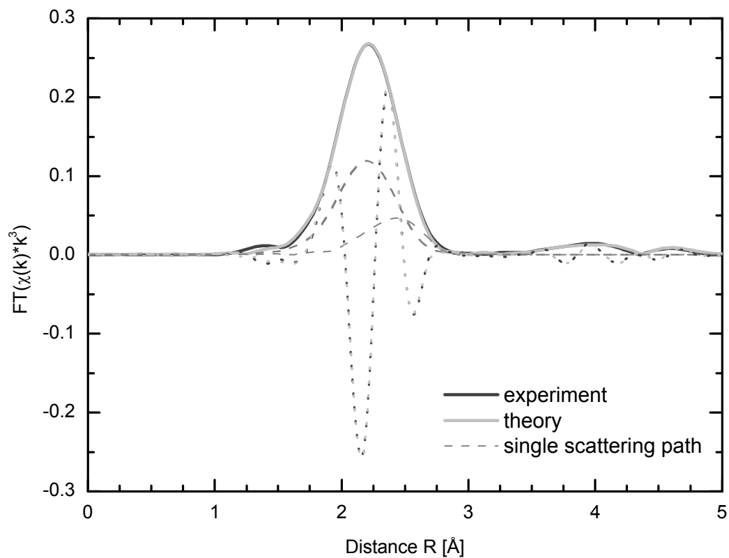
Figure 17: Experimental and theoretical Pd K edge FT(\chi(k) \cdot k^3) of Pd_3Ga_7 at 300 K.
