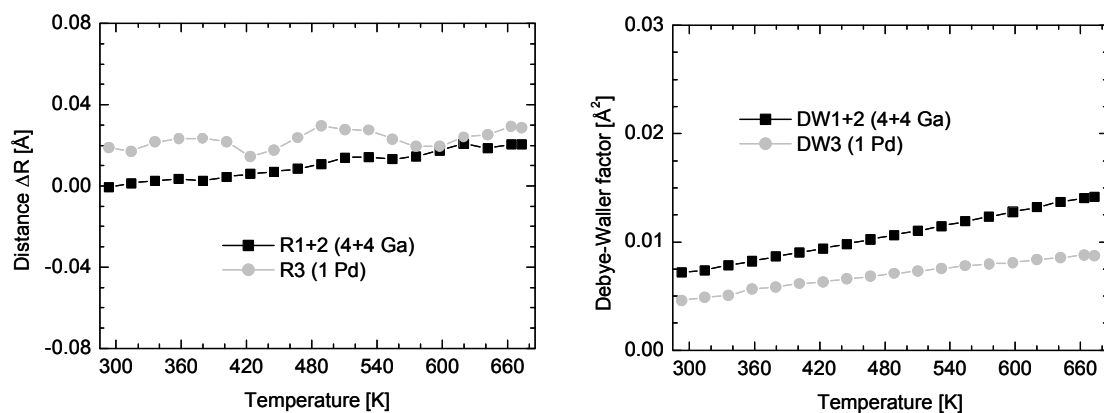
Figure 30: Evolution of selected relative Pd-Ga and Pd-Pd distances and Debye-Waller factors (right) of selected scattering paths of PdGa during thermal treatment of \text{Pd}_3\text{Ga}_7 in 50% hydrogen in helium from 323 K to 693 K obtained from analysis of the corresponding EXAFS spectra.
