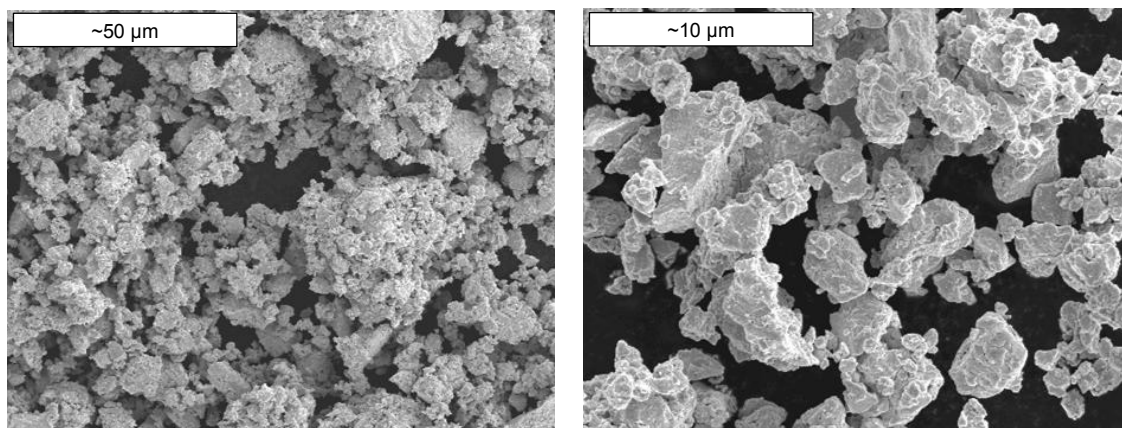
Figure 59: Scanning electron microscopy images of ball-milled \text{PdSn}_2 after heating in 50% hydrogen in helium to 573 K.
