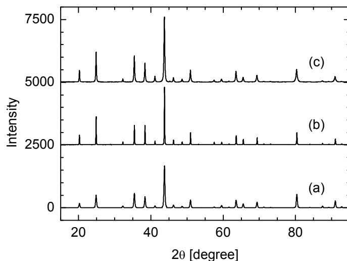
Figure 15: Experimental X-ray diffraction patterns of \text{Pd}_3\text{Ga}_7 (b) after grinding in a mortar and (c) after ball milling, together with a simulated pattern of \text{Pd}_3\text{Ga}_7 (a) [62].
