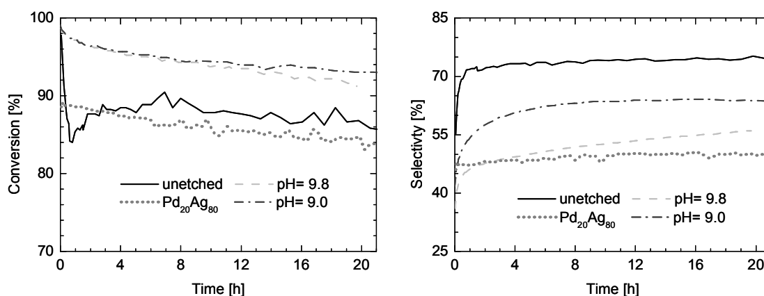
Figure 41: Conversion (left) and selectivity (right) of untreated PdGa (40 mg), PdGa chemically etched at pH= 9.8 (1.5 mg) and pH= 9.0 (5 mg), and Pd 20 Ag 80 (200 mg) in acetylene hydrogenation (isothermal at 473 under condition B).
