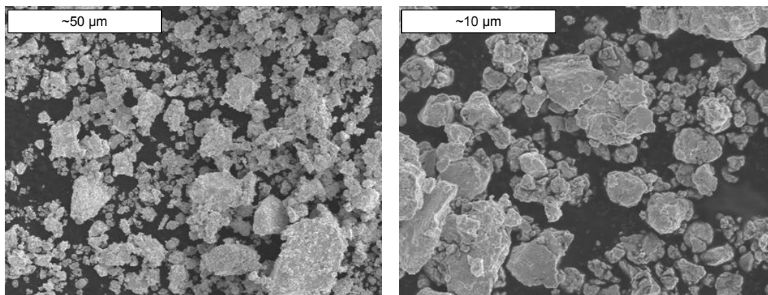
Figure 58: Scanning electron microscopy images of ball-milled \text{PdSn}_2 .
