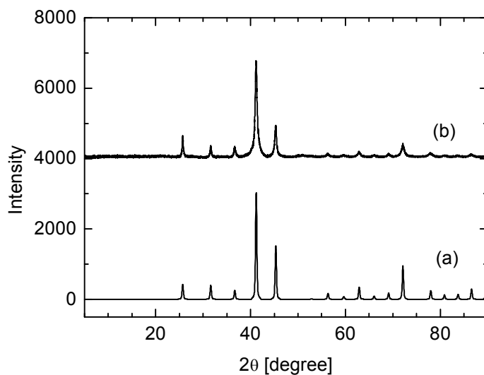
Figure 43: Experimental XRD pattern of PtPd 2 Ga 3 : simulated pattern (a) and after ballmilling (b).
