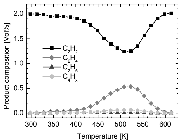
Figure 65: Product composition measured during hydrogenation of acetylene on PdSn 2 (100 mg) under condition A.
