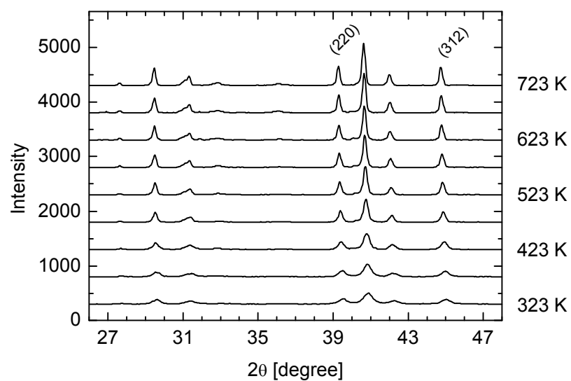
Figure 60: Evolution of X-ray diffraction pattern of PdSn 2 during thermal treatment from 323 K to 723 K in 50% H 2 + 50% He.
