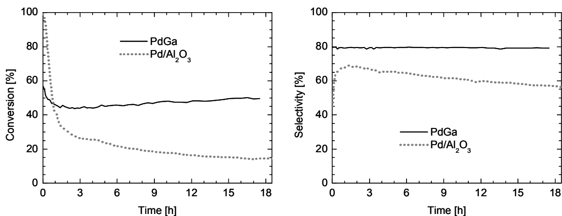
Figure 37: Conversion and selectivity of PdGa (50 mg) and of Pd/Al 2 O 3 (0.5 mg) in acetylene hydrogenation (isothermal at 393 K under condition A).
