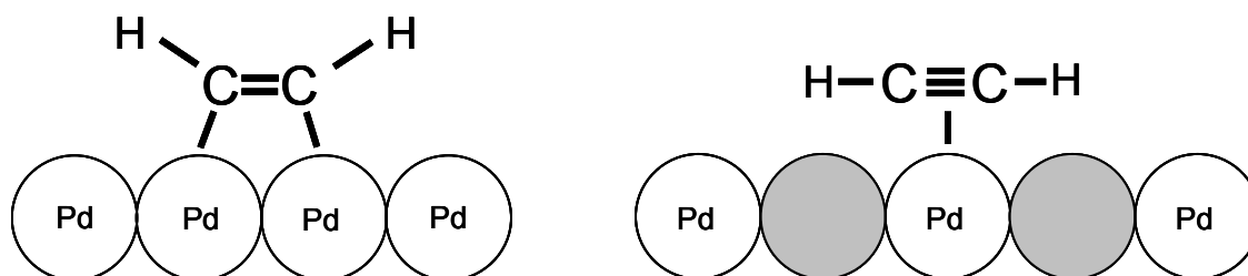
Figure 1: Di- \sigma bonded acetylene molecule to two neighbouring Pd atoms (left) and a weakly \pi -bonded acetylene molecule to an isolated Pd atom (right). Only the \pi -bonded acetylene is hydrogenated in high selectivity to ethylene.
