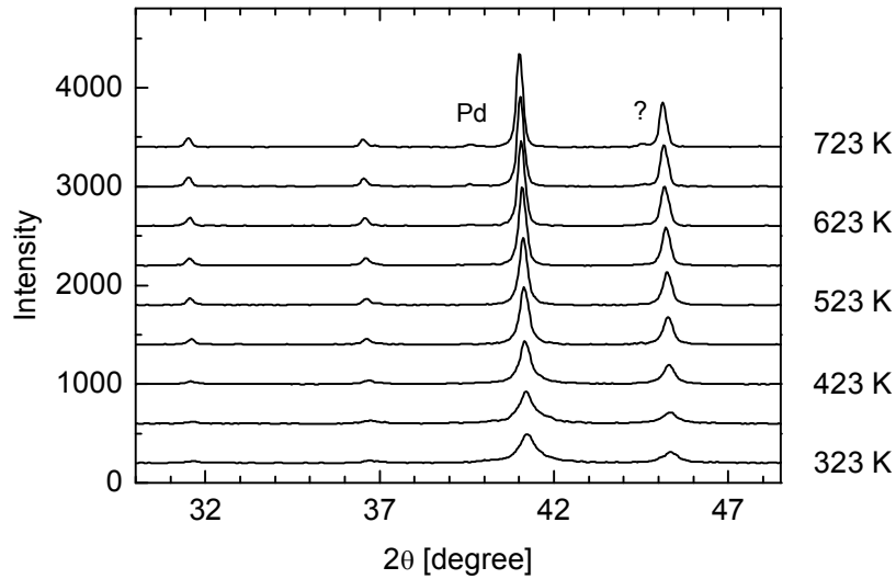
Figure 23: Evolution of in situ X-ray diffraction patterns measured during thermal treatment of PdGa in 20% oxygen in helium from 323 K to 723 K. Additional peaks at 674 K are due to the formation of Pd metal and an unidentified phase.
