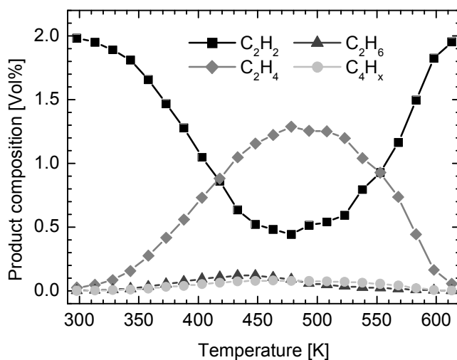
Figure 49: Product composition measured during hydrogenation of acetylene on PtPd 2 Ga 3 (60 mg) (2% C 2 H 2 + 4% H 2 , condition A).
