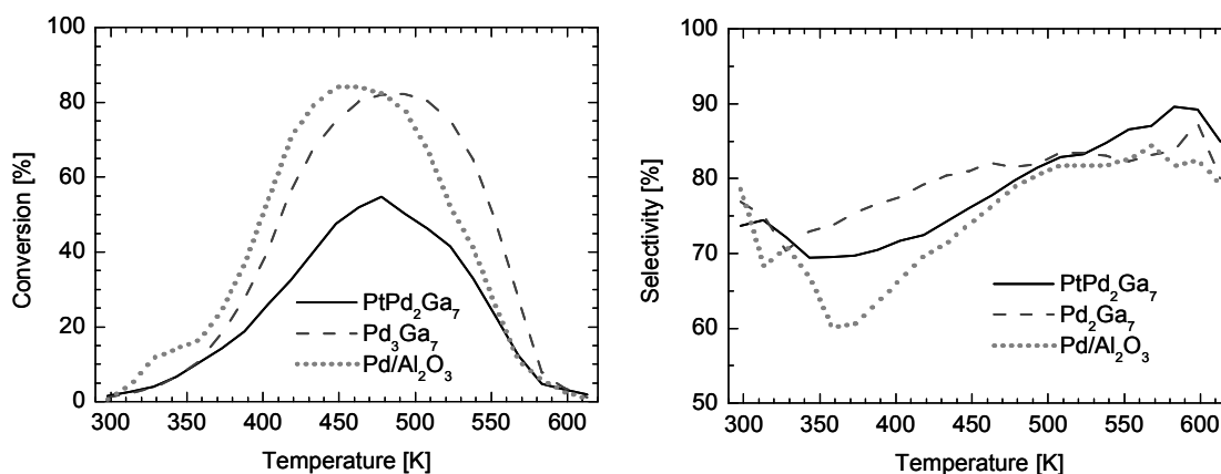
Figure 51: Conversion and selectivity measured during acetylene hydrogenation on PtPd 2 Ga 7 (120 mg), Pd 3 Ga 7 (100 mg) and Pd/Al 2 O 3 (0.5 mg) under reaction condition A.
