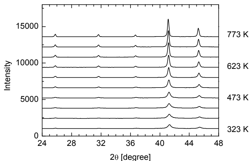
Figure 46: Evolution of in situ X-ray diffraction patterns of \text{PtPd}_2\text{Ga}_3 during thermal treatment from 323 K to 773 K in 50% \text{H}_2 + 50% He.
