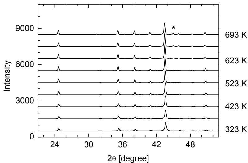
Figure 25: Evolution of in situ X-ray diffraction patterns measured during thermal treatment of \text{Pd}_3\text{Ga}_7 in 100% helium from 323 K to 693 K. Formation of \text{PdGa} at higher temperature is observable (*).
