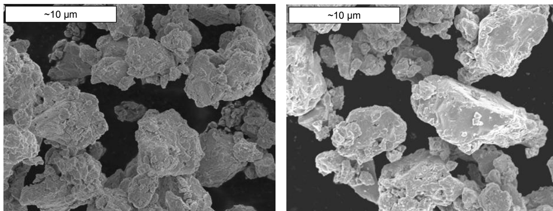
Figure 21: Scanning electron microscopy images of ball-milled \text{Pd}_3\text{Ga}_7 before (left) and after (right) heating in 50% hydrogen in helium to 573 K.
