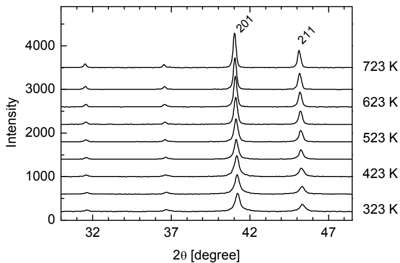
Figure 22: Evolution of in situ X-ray diffraction patterns measured during thermal treatment of PdGa in 50% hydrogen in helium from 323 K to 723 K.
