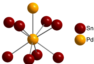
Figure 7: Coordination sphere of Pd atoms in PdSn 2 .
