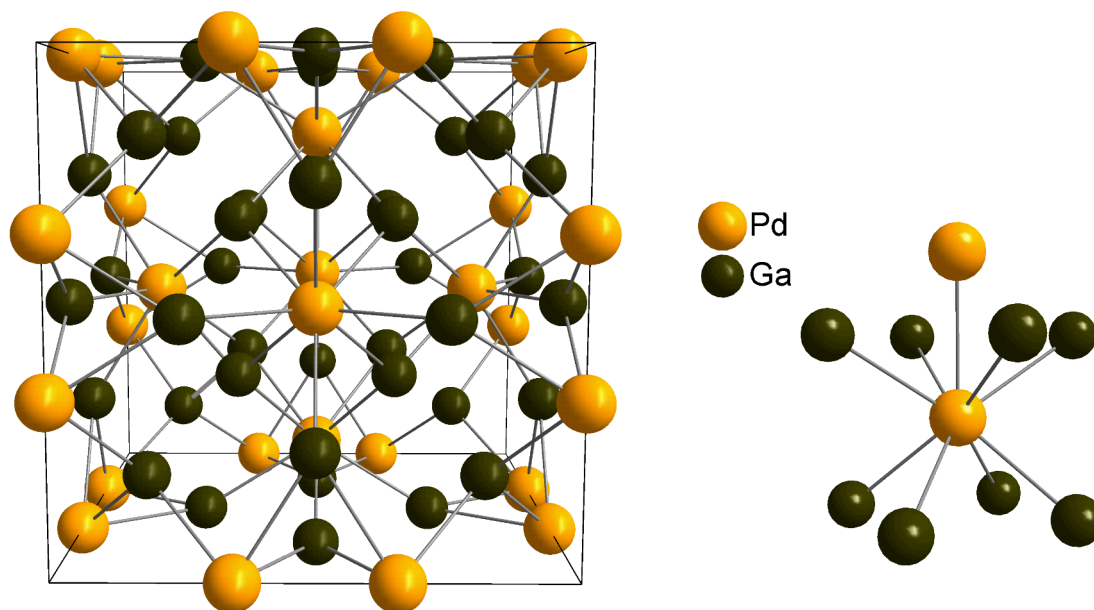
Figure 5: Unit cell of \text{Pd}_3\text{Ga}_7 and coordination sphere of Pd atoms in \text{Pd}_3\text{Ga}_7 .
