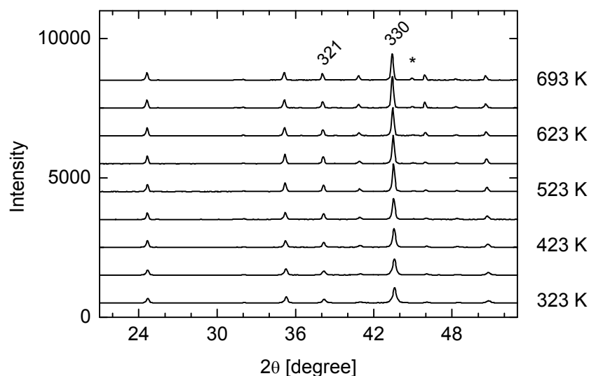
Figure 24: Evolution of in situ X-ray diffraction patterns measured during thermal treatment of \text{Pd}_3\text{Ga}_7 in 50% hydrogen in helium from 323 K to 693 K. Formation of PdGa at higher temperature is observable (*).
