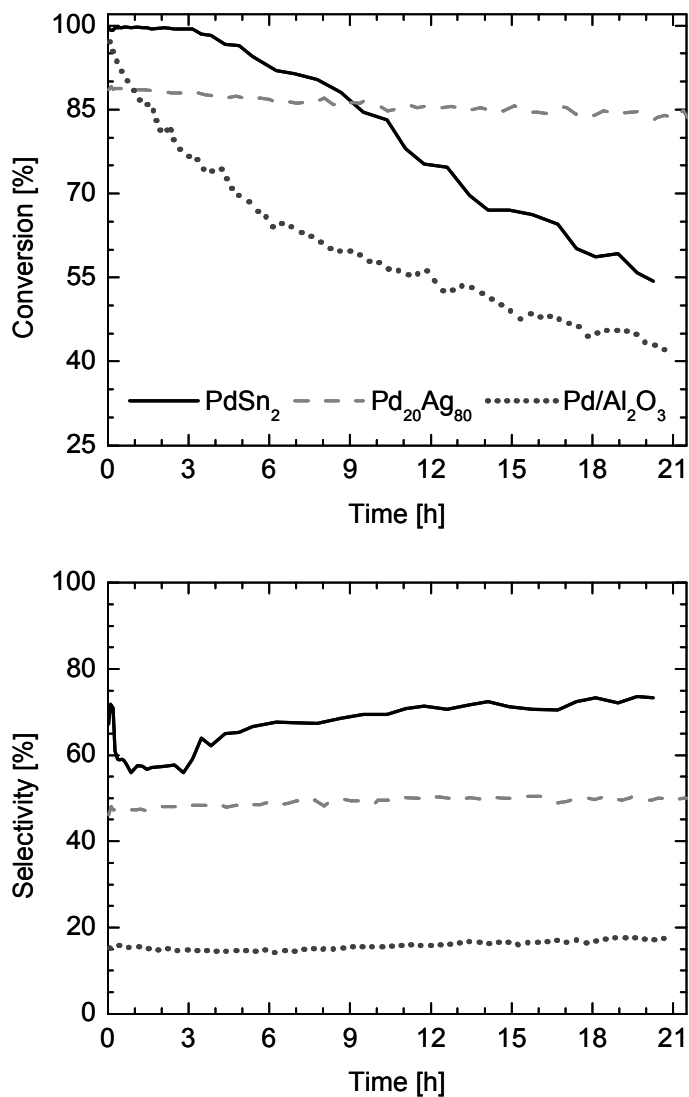
Figure 66: Acetylene conversion and corresponding selectivity of chemically etched (NaOH + EDTA) \text{PdSn}_2 (85 mg), \text{Pd}/\text{Al}_2\text{O}_3 (0.15 mg) and \text{Pd}_{20}\text{Ag}_{80} (200 mg) isothermal at 473 K (condition B).
