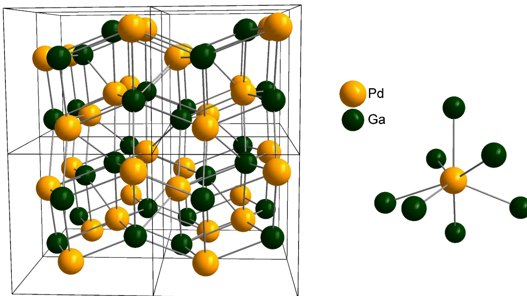
Figure 4 : 2x2x2 unit cell of PdGa and coordination sphere of Pd atoms in PdGa.
