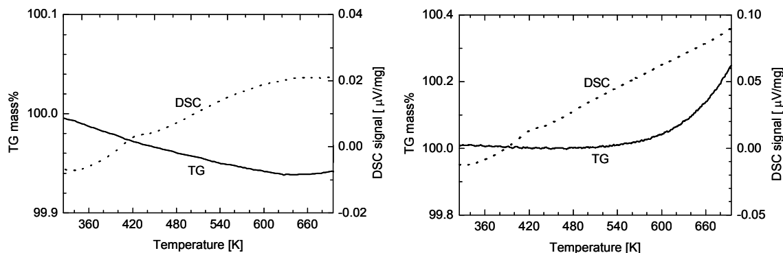
Figure 19: Relative mass (TG) (solid) and DSC signal (dotted) during thermal treatment (300 K – 693 K at 6 K/min) of \text{Pd}_3\text{Ga}_7 in 50% hydrogen in He (left) and in 50% oxygen in He (right).
