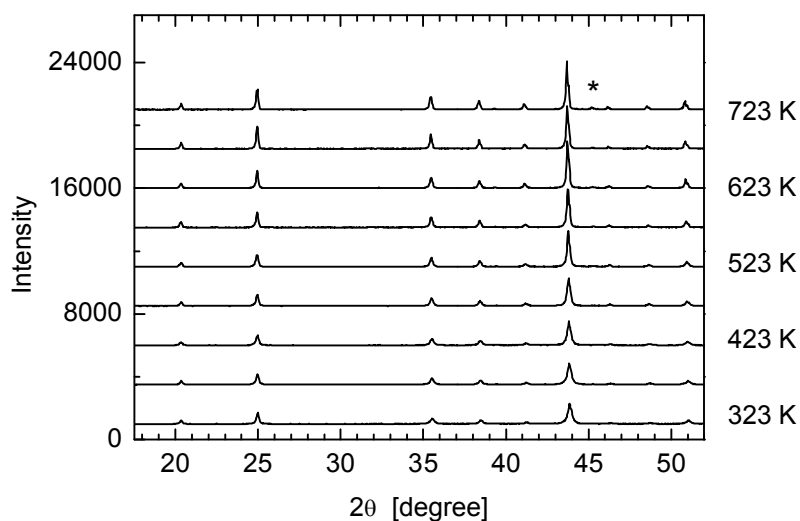
Figure 47: Evolution of in situ X-ray diffraction patterns of \text{PtPd}_2\text{Ga}_7 during thermal treatment from 323 K to 723 K in 50% \text{H}_2 + 50% He. Formation of \text{PtPd}_2\text{Ga}_3 at higher temperature is observable (*).
