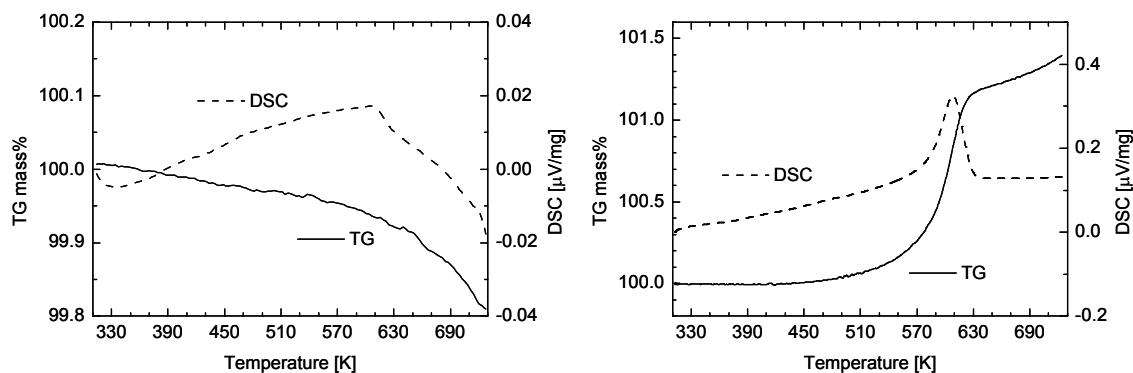
Figure 57: Relative mass (TG) (solid) and DSC signal (dashed) during thermal treatment of \text{PdSn}_2 in 50% hydrogen in helium (left, 300 K – 723 K at 6 K/min) and in 50% oxygen in He (right, 300 K – 723 K at 6 K/min).
