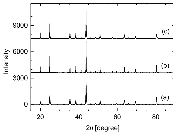
Figure 44: XRD pattern of PtPd 2 Ga 7 : Simulated pattern (a), experimental pattern after grinding in a mortar (b) and after ballmilling (c).
