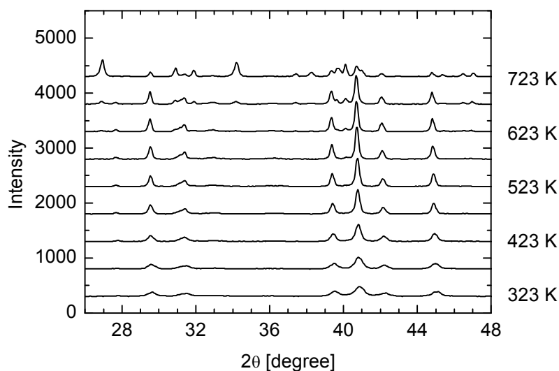
Figure 62: Evolution of X-ray diffraction pattern of \text{PdSn}_2 during thermal treatment from 323 K to 723 K in 100% helium.
