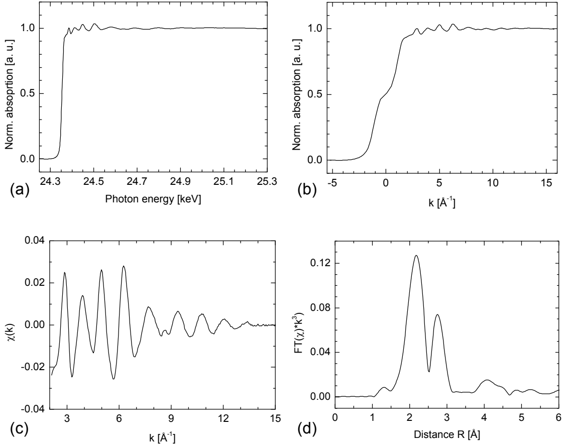
Figure 12: An example for EXAFS data processing: (a) background corrected and normalised absorption spectrum of PdGa, (b) after transformation into k-space, (c) extracted \chi(k) and (d) after Fourier transformation of the \chi(k) .
