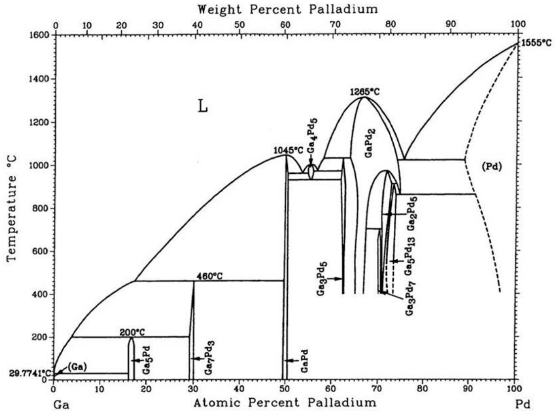
Figure 3: Phase diagram gallium-palladium [58].
