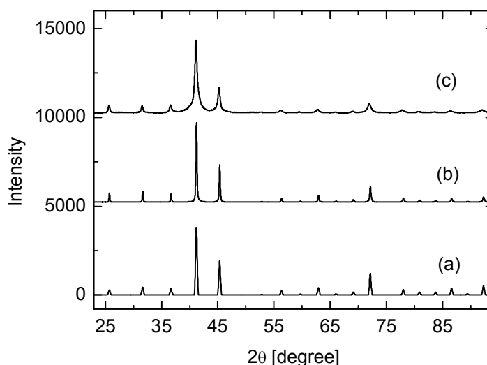
Figure 14: Experimental X-ray diffraction patterns of PdGa (b) after grinding in a mortar and (c) after ball milling, together with a simulated pattern of PdGa (a) [62].
