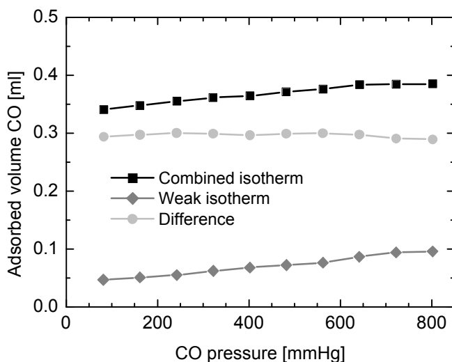
Figure 34: CO chemisorption on Pd/Al 2 O 3 (5%wt) after hydrogen pre-treatment at 473 K. First adsorption isotherm (combined) contains the chemisorbed and physisorbed part of CO on Pd/Al 2 O 3 . Second isotherm was measured after evacuation and resulted in the weak isotherm (only physisorbed CO). The difference of combined and weak isotherm can be used for calculation of the chemisorbed part of the CO on Pd/Al 2 O 3 .
