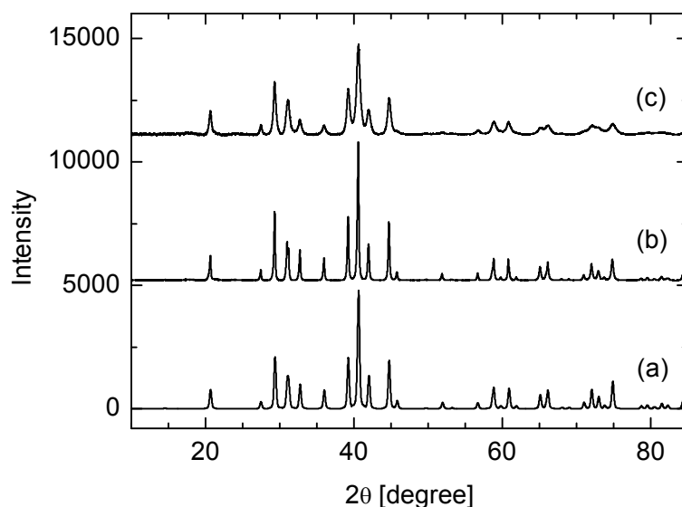
Figure 55: Experimental X-ray diffraction patterns of PdSn 2 (b) after grinding in a mortar and (c) after ball milling, together with a simulated pattern of PdSn 2 [65].
