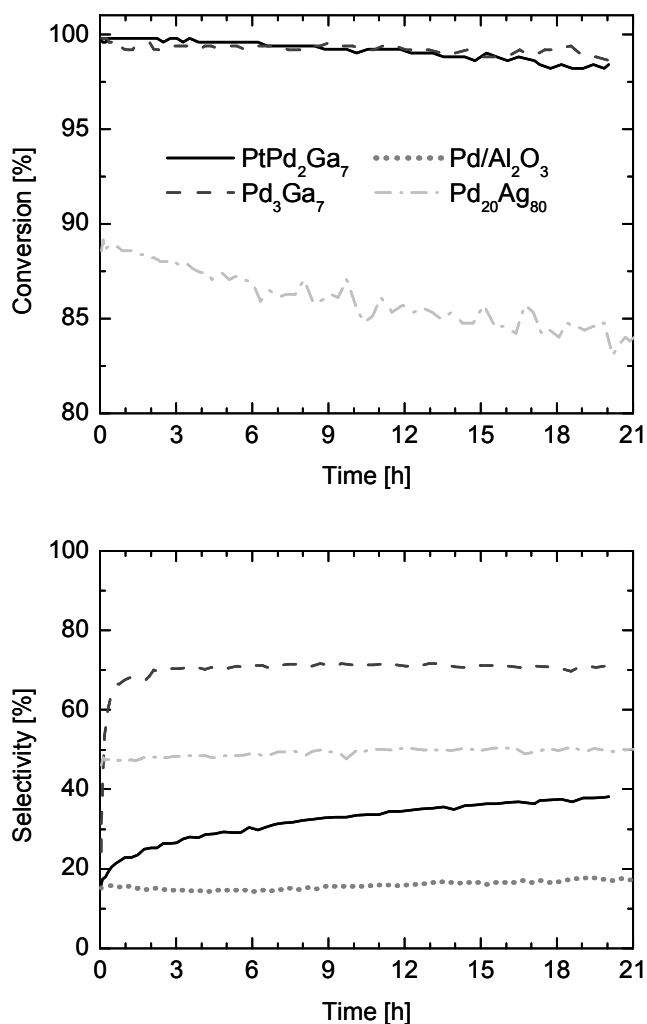
Figure 53: Acetylene conversion and selectivity of \text{PtPd}_2\text{Ga}_7 (100 mg), \text{Pd}_3\text{Ga}_7 (100 mg), \text{Pd}/\text{Al}_2\text{O}_3 (0.15 mg, only selectivity) and \text{Pd}_{20}\text{Ag}_{80} (200 mg) isothermal at 473 K (condition B).
