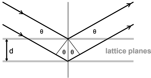
Figure 8: Bragg reflection of X-rays at lattice planes.
