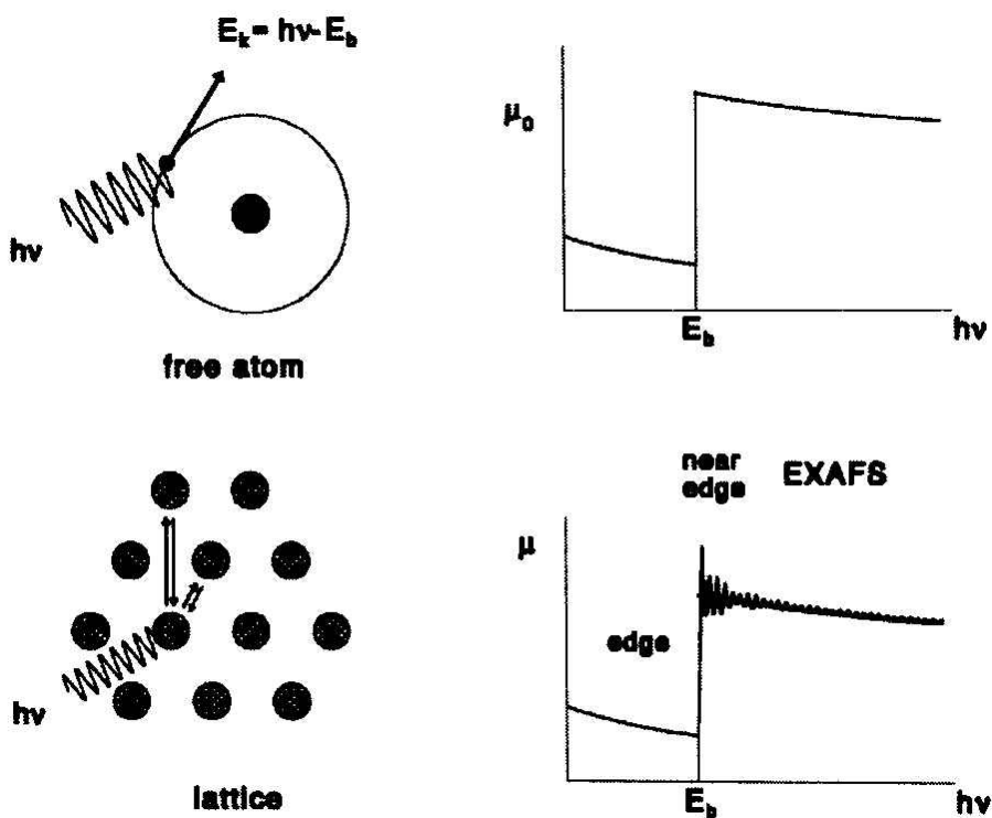
Figure 10: Absorption of X-rays as a function of photon energy by a free atom and an atom in a lattice. The fine structure is due to interference of outgoing and backscattered electron waves [80].
