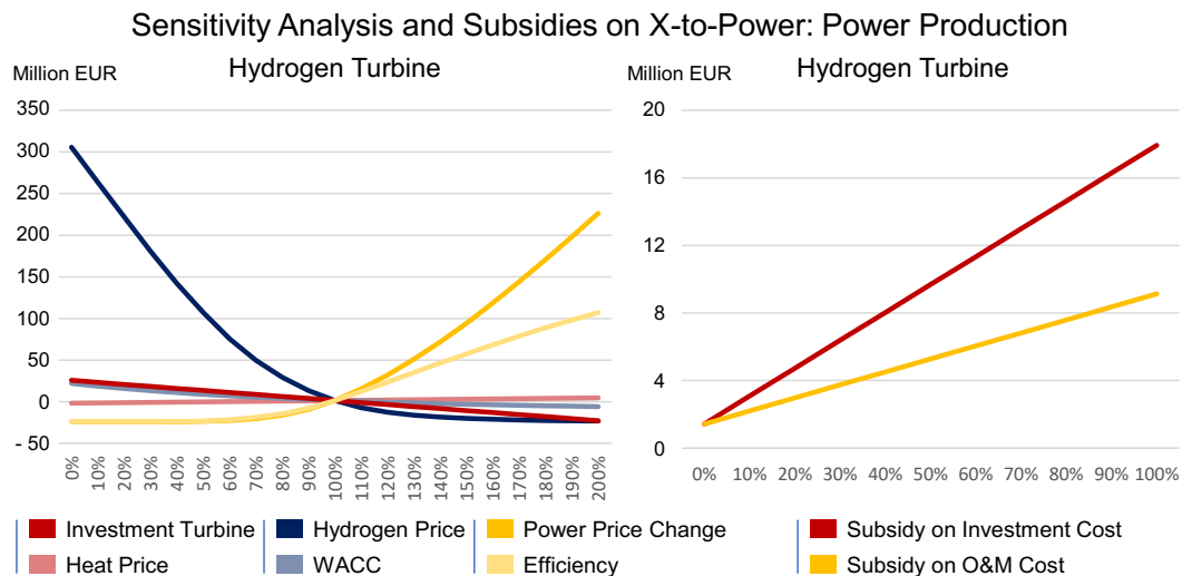
Figure 10: Sensitivity of the NPV (left) and the impact of subsidies on the NPV (right) of the XtP business model
